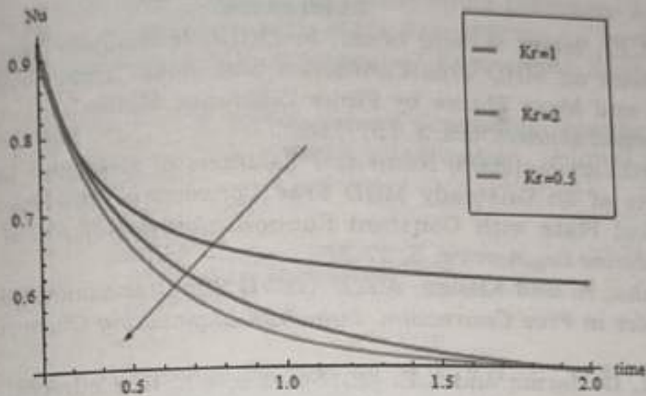
Figure 20. Nusselt number when Sc = 0.22, Pr = 0.7, Du = 2, Q = 1
