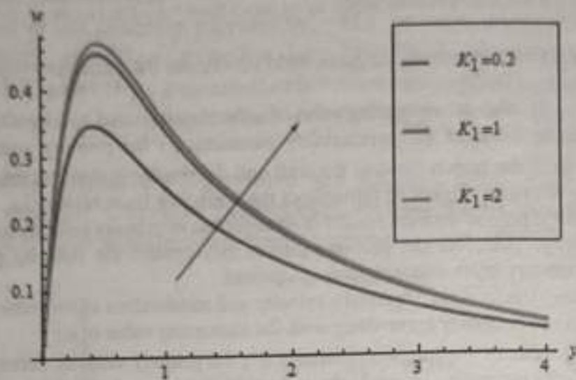
Figure 5. Secondary velocity profiles when
