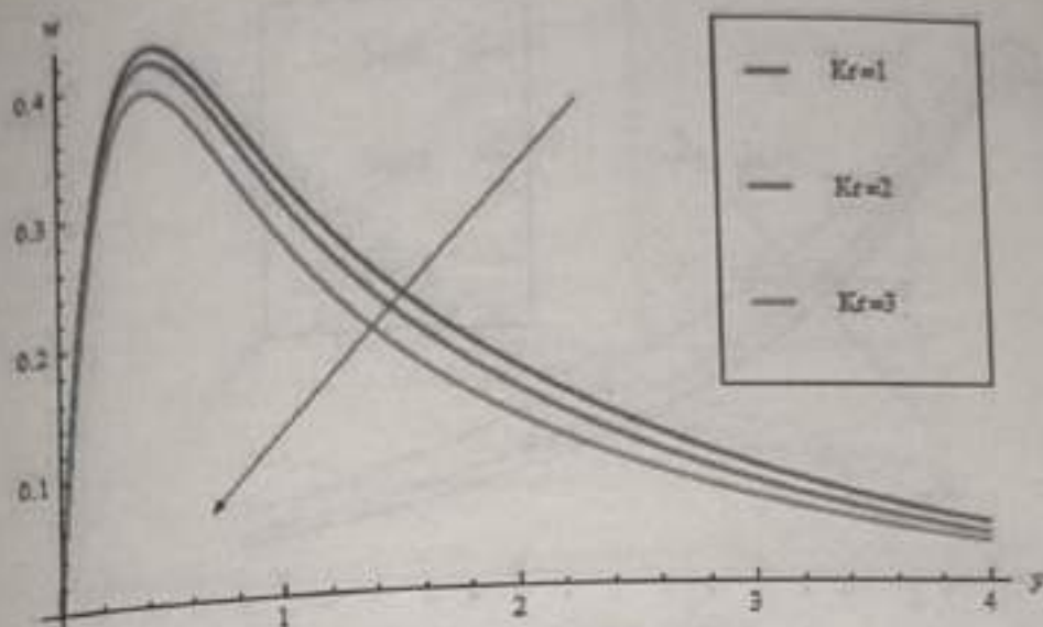
Figure 11. Secondary velocity profiles when Du = 2, K^2 = 5, Gr = 6, Sc = 0.22, Pr = 0.7, Gm = 5, t = 1, m = 0.5, K_1 = 0.5
