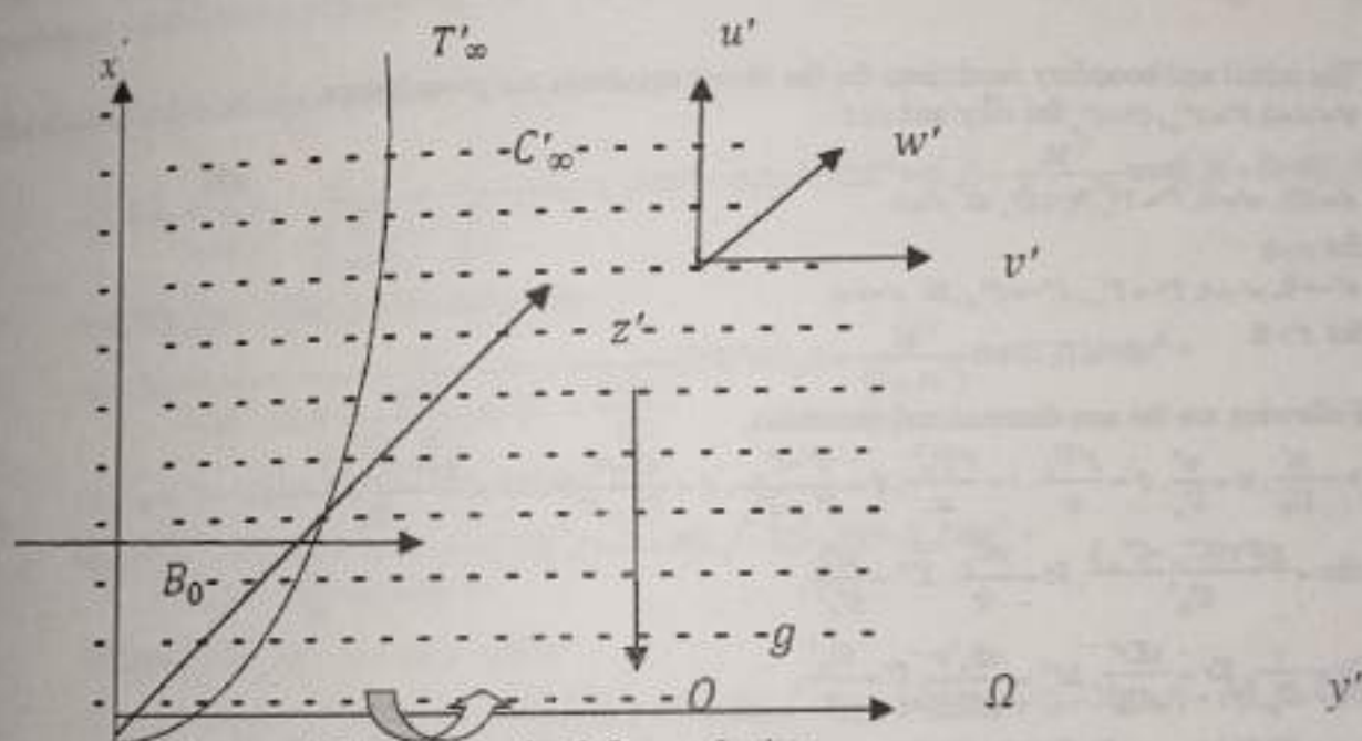
Figure 1. Mathematical formulation
