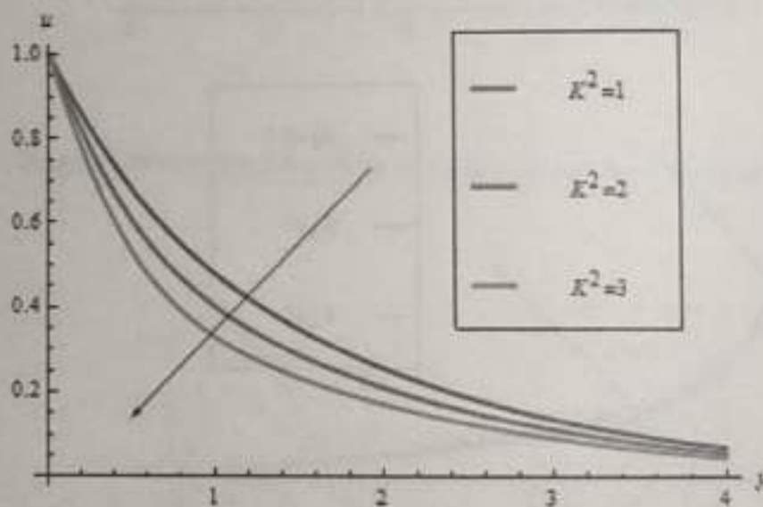
Figure 6. Primary velocity profiles when
