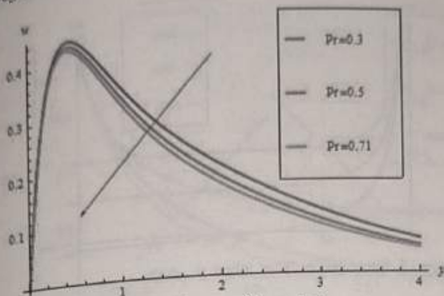
Figure 15. Secondary velocity profiles when Sc = 0.22, K^2 = 5, Gr = 6, Gm = 5, Du = 2, Kr = 1, t = 1, m = 0.5, K_1 = 0.5
