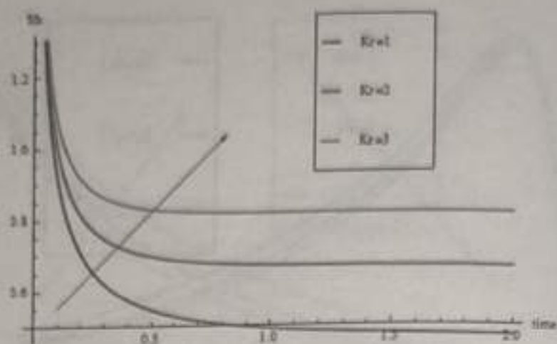
Figure 17. Sherwood number when Sc = 0.22
