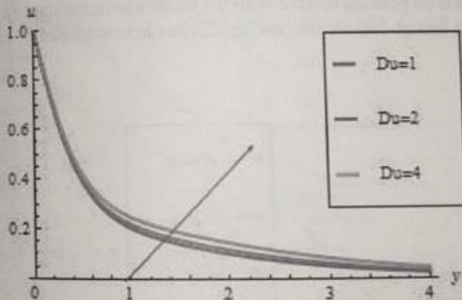
Figure 12. Primary velocity profiles when Sc = 0.22, K^2 = 5, Gr = 6, Gm = 5, Pr = 0.7, Kr = 1, t = 1, m = 0.5, K_1 = 0.5
