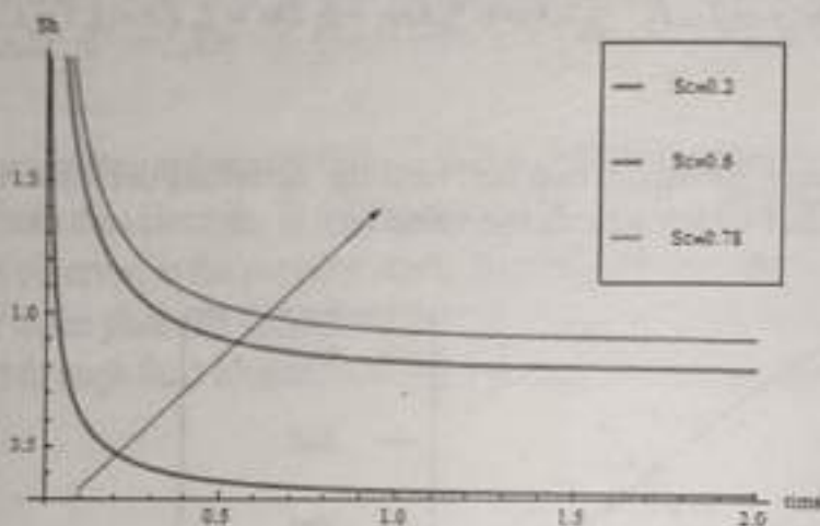
Figure 18. Sherwood number when Kr = 1
